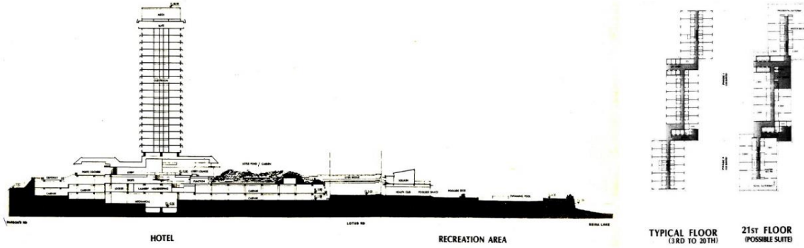
Perspectives, Cross-sectional & Floor Layout Sheets as per Project Plans for Colombo Hilton Hotel
